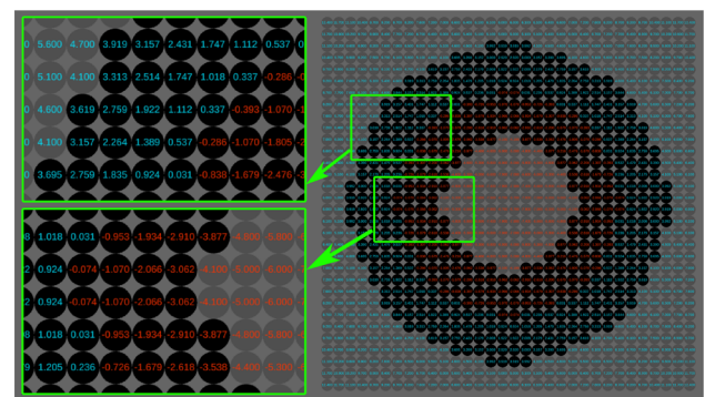
Fig. 6 A slice from a 32 3 SDF volume of a sphere. The red text means negative SDF values. The blue text means positive SDF values. The black cell means Group A: floating-point data with 3 decimal places in \{-4.001, \dots, 4.001\} . The gray cell means Group B: the rest of 65,535 floating-point data in \{-2880.6, \dots, -4.1\} \cup \{4.1, \dots, 2880.6\}
