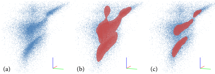
Figure 4.10: CloudLasso being applied to a 3D scatter plot; data from a subset of the milliMillennium dataset [De Lucia and Blaizot, 2007] (showing the dimensions virial radius, R-I color, and low X-ray luminosity); (a) original 3D scatter plot, (b) initial CloudLasso selection, (c) after interactive threshold adjustment.
