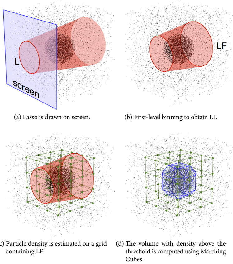
Figure 4.4: Main steps of the CloudLasso selection algorithm.
