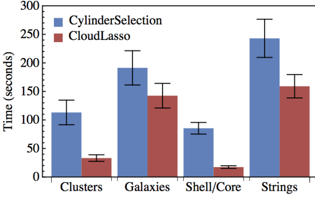
Figure 4.8: Mean completion times for the user study tasks. Error bars represent 95% confidence intervals.
