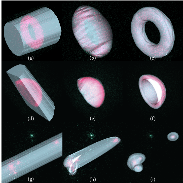
Figure 4.9: Comparison of CylinderSelection (left column), TeddySelection (middle column), and CloudLasso (right column) in three different examples. From top to bottom: selection of a torus-shaped structure, a concave hemispherical shell (i. e., an empty, thickly-walled bowl), and two clusters from an astronomical N-body simulation. The three selections in each example are made from the same viewpoint with respect to the particles and the result is viewed from roughly the same direction.
