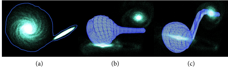
Figure 4.1: Problem with Teddy-like placement of a selection mesh in the 3D data space: (a) lasso in the original view direction, drawn from a ‘top-down’ view; (b) selection mesh after a 90^\circ rotation, placed at constant depth—the mesh does not wrap around the data; (c) depth adjusted to local average particle depth—the mesh still does not properly wrap around the data due to only being parameterized by the drawn lasso.
