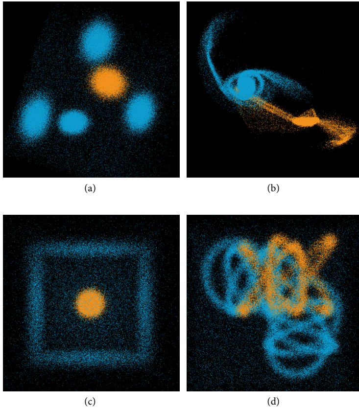
Figure 4.7: Four tasks: (a) five simple particle clusters, (b) two galaxies, (c) cubic shell and central core, and (d) three intertwined figure-eight knots.
