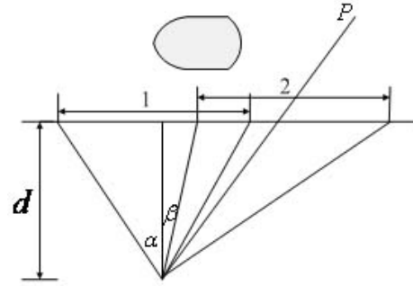
Figure 4. Geometry correction
