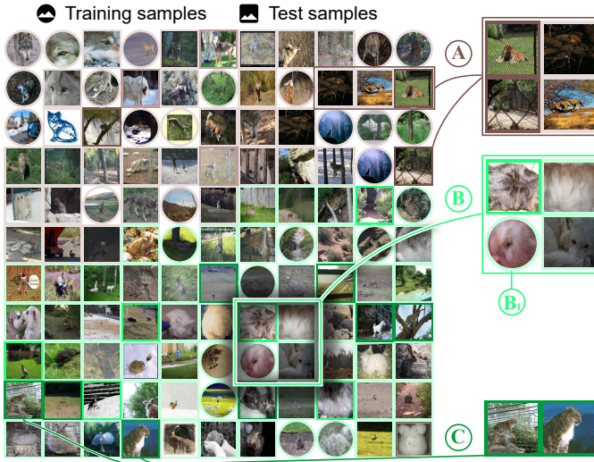
Fig. 10: After zooming into region Fig. 1D, more samples with high OoD scores are identified (A and C). Our layout also reveals that some samples with only part of an animal (B) are misclassified as “rabbit” due to a low-quality training sample with only the hair of a rabbit ( B_1 ).
