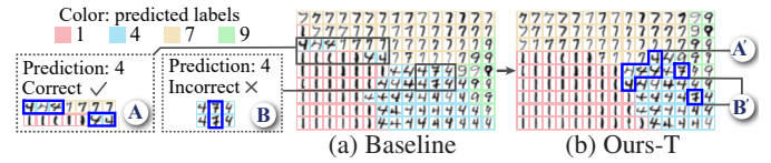
Fig. 9: Compared with the baseline (a), the samples predicted as “4” (A and B) are merged into the cluster of “4” in our layout (b).
