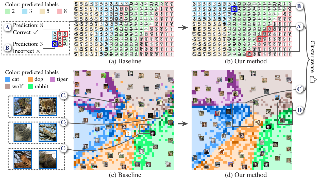
Fig. 1: Top: compared with the baseline (a) that only optimizes proximity, our method (b) places the samples that are predicted as “8” (A) in the cluster of “8.” Bottom: compared with the baseline (c), our method (d) groups the dark blue cells C_1 - C_3 in region C' .
