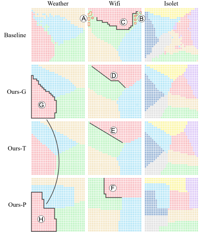
Fig. 8: Comparison of the layouts generated by the baseline (OoDAnalyzer [9]), Ours-G, Ours-T, and Ours-P. Using our methods, samples that fall into other clusters (A and B) are placed into their corresponding clusters, and irregular boundaries between different clusters (C) become regular (D, E, and F). Boundaries in Ours-G and Ours-T contain many slanted segments (D, E, and G), while boundaries in Ours-P mainly consist of horizontal and vertical segments (F and H).
