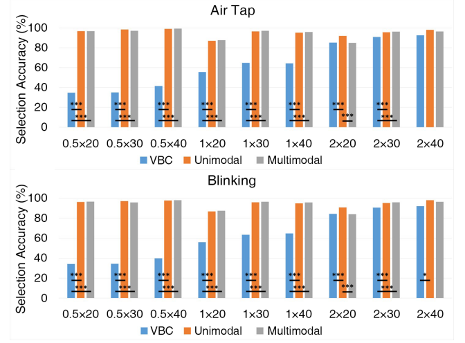
Figure 9: Selection accuracy of the three techniques in air tap (TOP) and blinking (BOTTOM) conditions for each W \times A combination.
