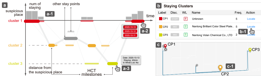
Figure 5: (a) The transportation activity chart depicts the moving and staying activities of trucks. It encodes the spatial and temporal contexts of a trajectory in a 2D space. The polyline becomes bold when being hovered or selected. (b) The staying cluster panel lists the clustered places in the historical trajectories. (c) The activity view is coordinated with the spatial view.
