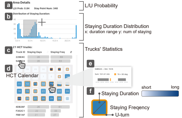
Figure 4: The temporal view in Helium. (a) The L/U probability. (b) The distribution of stay points on staying duration. (c) Statistics about the related HCT trucks. (d) When users select one truck, a HCT calendar displays details about the truck’s staying behaviors per day. (e) When users hover over one date, a card presents the staying events within that day. (f) The visual encoding of the calendar unit.
