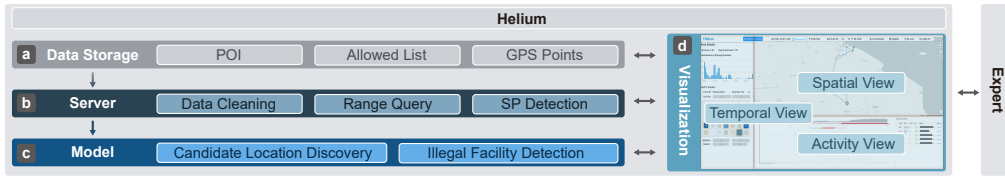
Figure 2: The system architecture of Helium. Helium consists of four modules, namely, (a) data storage, (b) server, (c) model, and (d) visualization. Experts can visually analyze suspicious places in Helium through flexible interactions.
