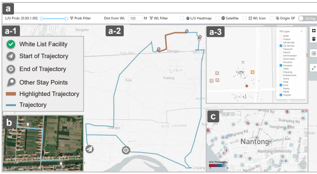
Figure 3: The spatial view includes (a) a street map with layer configurations, (b) a satellite map, and (c) a L/U probability heatmap. In the street map, the system provides (a1) stay point markers, (a2) original GPS locations, and (a3) the POI configuration panel.
