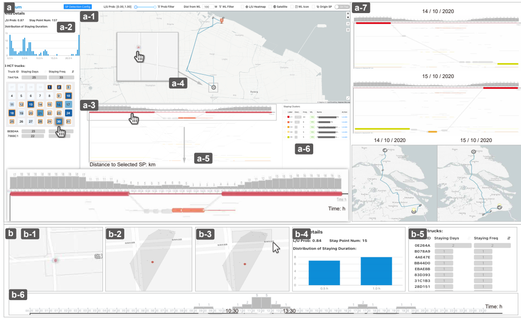
Figure 6: Two case studies about (a) an in-depth analysis of suspicious places and (b) reconsidering model results. (a) In the first case study, EA investigated the HCT truck behaviors through the coordinated spatial and activity views and further judged the suspicious place as an illegal facility. (b) In the second case study, after exploring the system, EB laid down a fake positive place detected by the automatic model.
