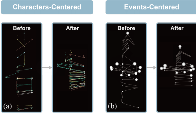
Fig. 4. Result of storyline layout optimization along time axis: (a) Character-Centered Perspective and (b) Event-Centered Perspective.
